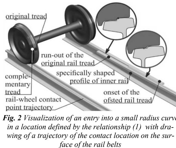
Fig. 2 Visualization of an entry into a small radius curve in a location defined by the relationship (1) with drawing of a trajectory of the contact location on the surface of the rail belts
