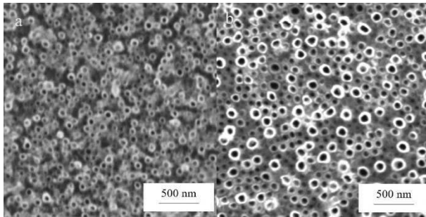
Fig. 2 nanostructures prepared at a) 20 V; b) 30 V after heat treatment
